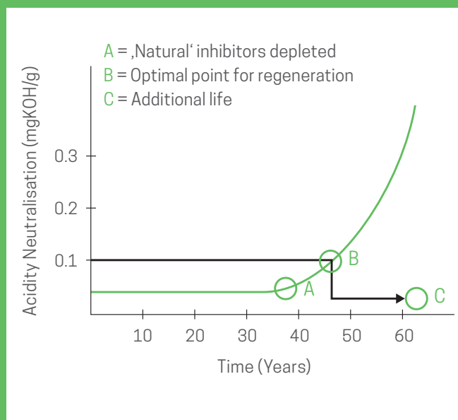
Acidity over time
