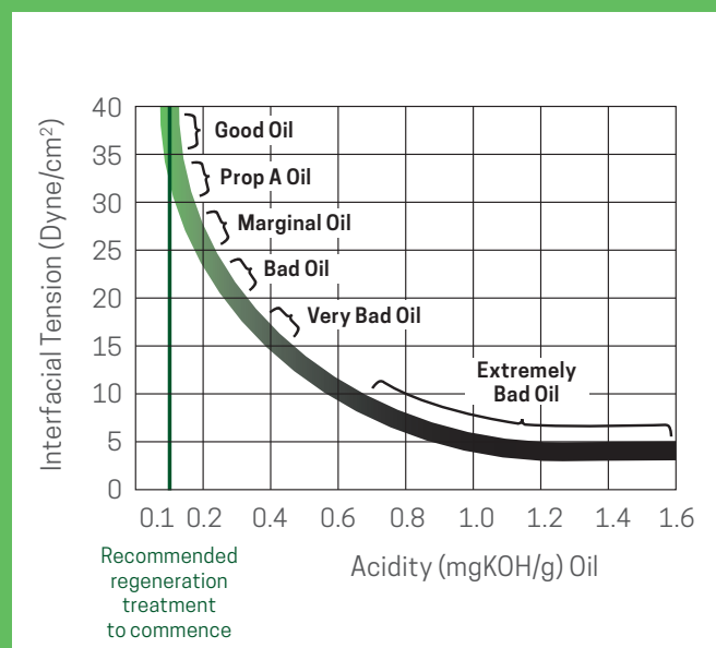
Comparison of neutralisation value versus interfacial tension
