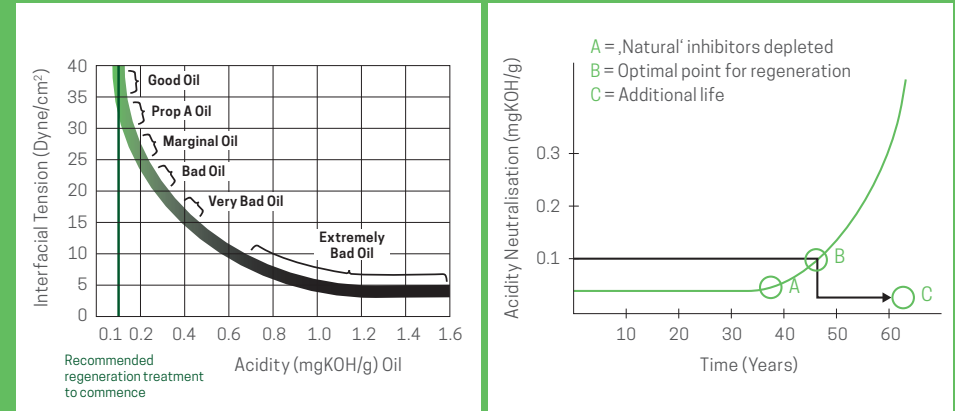
Comparison of neutralisation value versus interfacial tension
